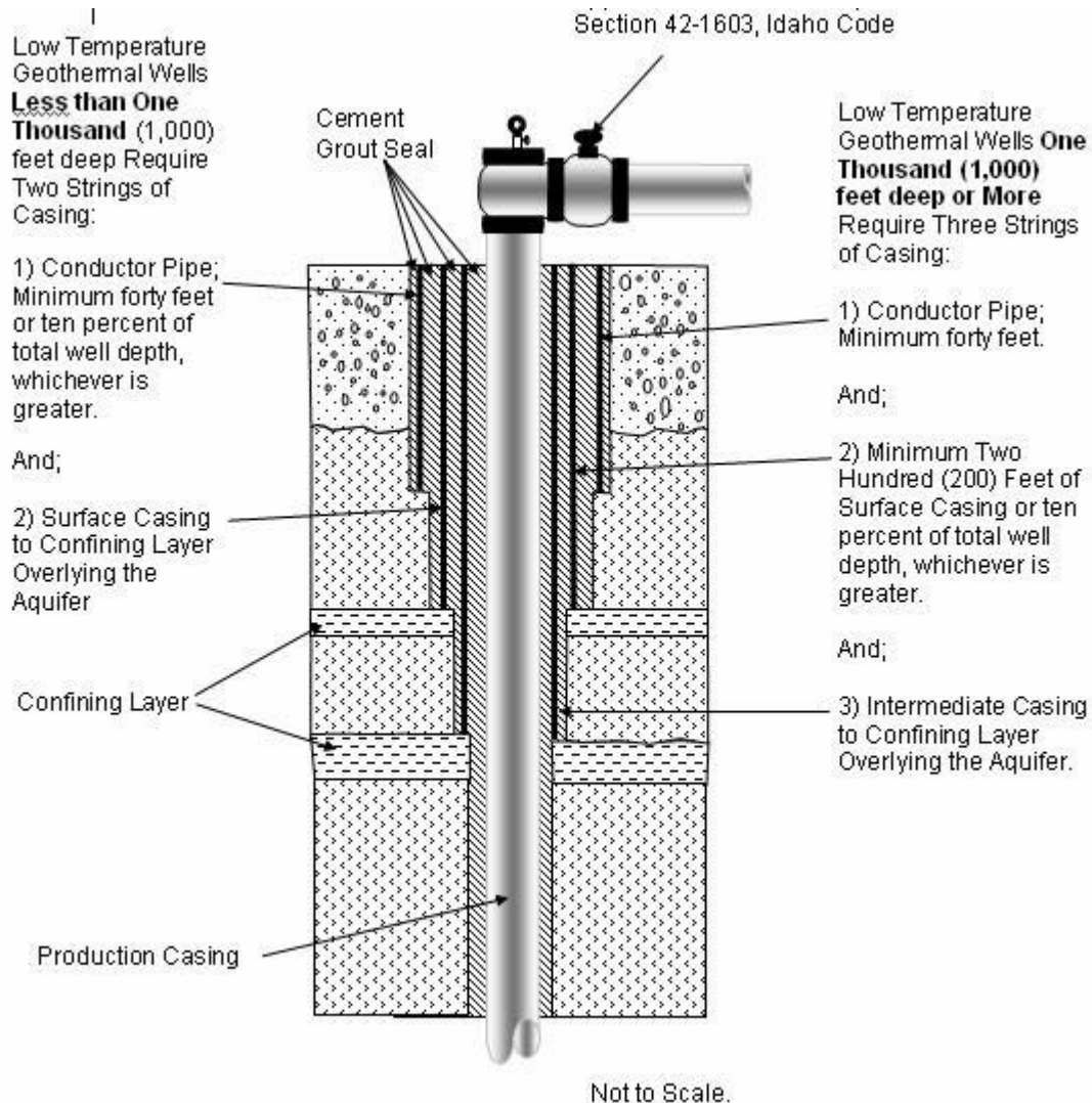
Figure 13. Casing Segments for Low Temperature Geothermal Wells.
