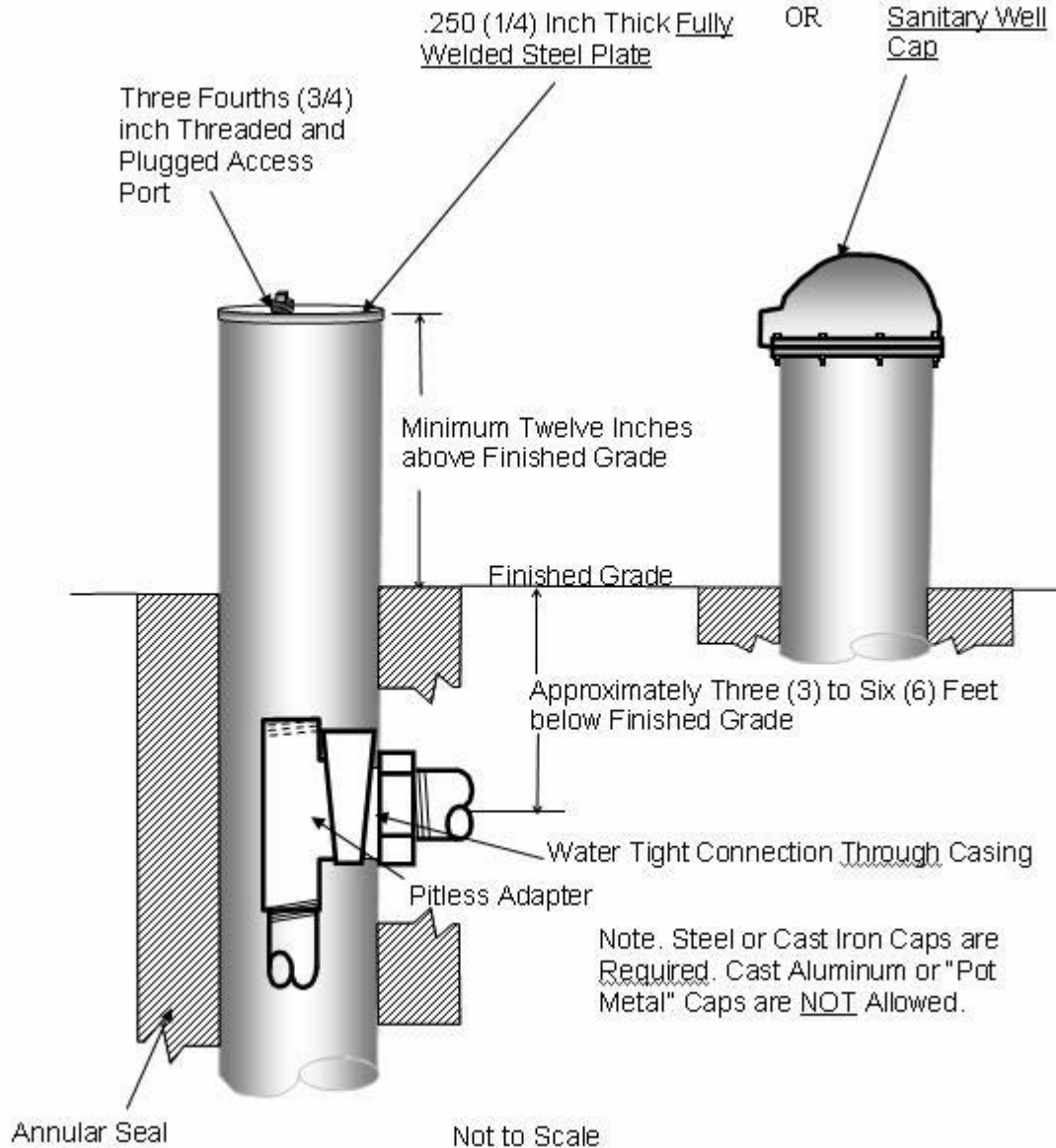
Figure 12. Well Cap and Access Port.
