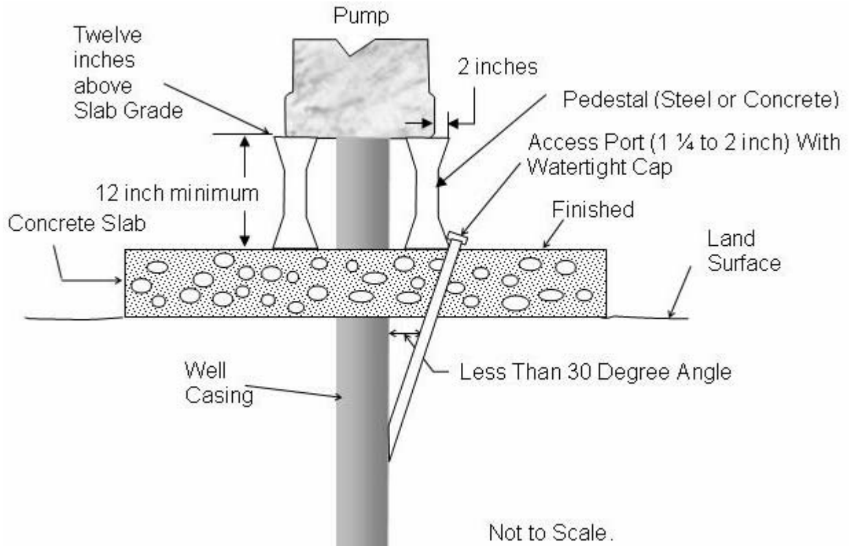
Figure 01. Concrete Slabs and Finished Grade.
